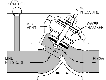
VALVE OPEN
