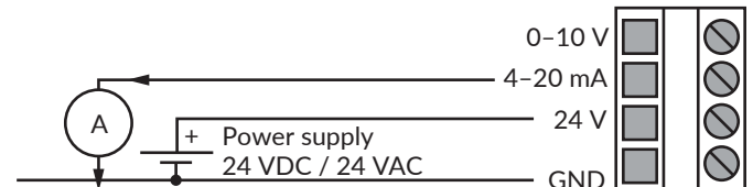
Figure 2b - Wiring diagram 4-20 mA output
